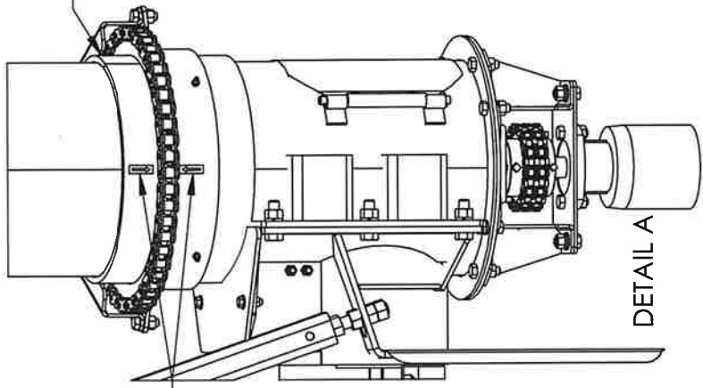
ARROWDECAL #76768 (STOP POSITION)
