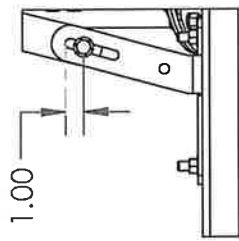
DETAIL E SCALE 1 : 10 TYPICAL FRONT & REAR MOUNTS
